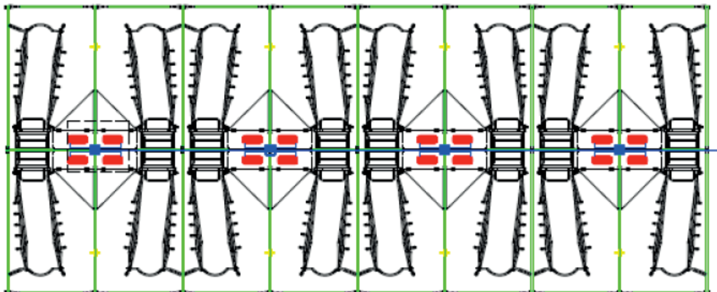
Installation of 16 Aniheater® with 8 Dual Controllers.
