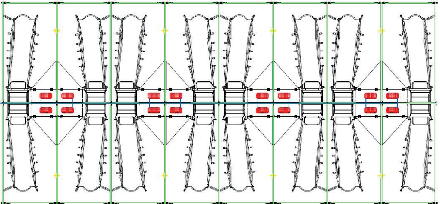
Installation of 16 Aniheater® with one Multi Controller A16.
